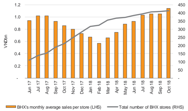
Figure 1: Our monthly performance tracking of BHX suggests improving store-level productivity and only gradual footprint expansion
